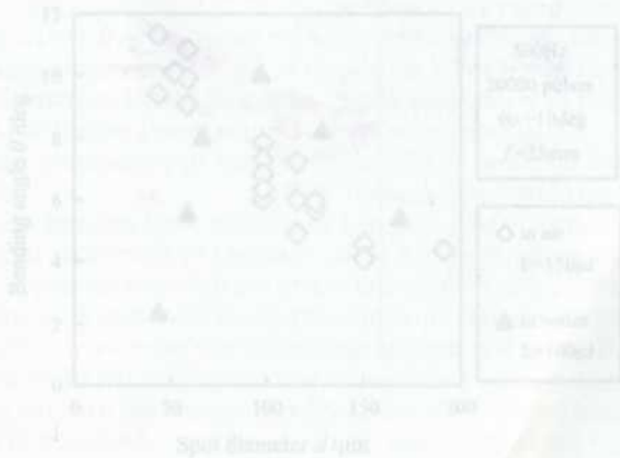
Fig. 10. Relationship between bending angle and spot diameter
